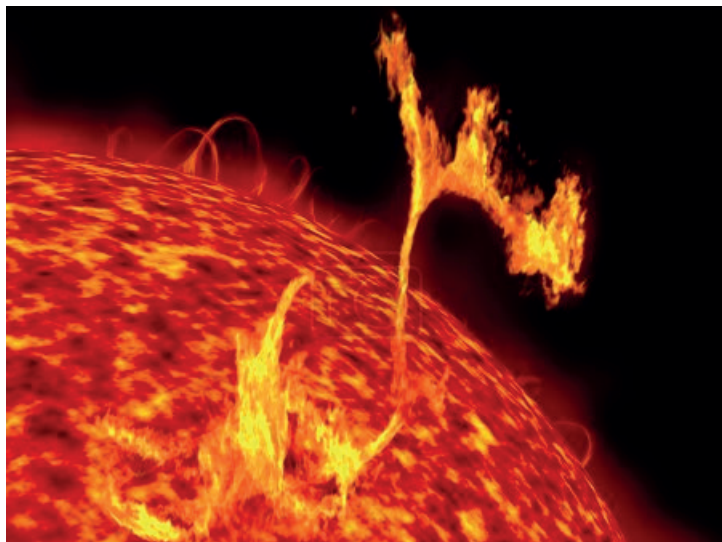
Рис. 8. Вспышка на Солнце ( https://photogenica.ru/preview-DP.php?directZoom=0EtGQXdwRXcya1MrVWEvUEVtQkRUREtNaDVDQlhhN0pBcWtTTUw0TXA3N2pzejVKOX11Y0hTcEdsUnBpNHNicGdHUURZY01FQkVQRjFNV0JqelpqdHNUWnRWQTFMVnNxUVFzQ25YM3hLZ1RDdUJSK2ZLYUodHNjd1hBRmYwcXdyMG5FTlduYUpRcjgyM3R5Q3ZWbVnPT0=&hash=b402b20aed02f060c4b9ed61f7738a841650b30ee34ba6c849322c1164b25d4 )
